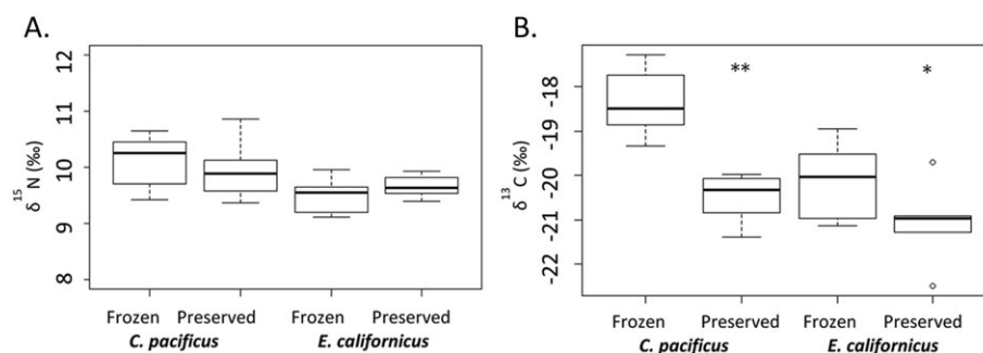
FIGURE 3 Bulk (A) \delta^{15}\text{N} and (B) \delta^{13}\text{C} values from the copepods Calanus pacificus and Eucalanus californicus , where paired samples were frozen or formaldehyde-preserved for 24–25 years. Mean \pm 95% SD. An asterisk (*) indicates significant differences with p < 0.05 and ** indicates p < 0.01
