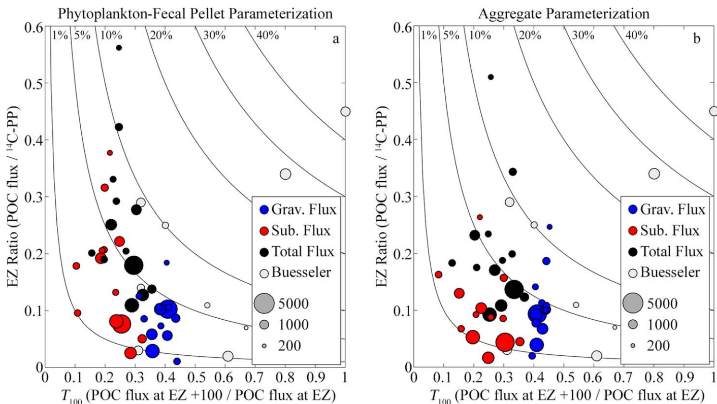
Fig. 9. Plot of EZ ratio (POC flux at the base of the EZ/ 14 CPP) vs. T_{100} (POC flux at 100 m below EZ/POC flux at EZ) for PFP parameterization (a) and Agg parameterization (b). Size of circle is proportional to primary productivity ( \text{mg C m}^{-2} \text{d}^{-1} ). Blue symbols are gravitational flux. Red symbols are for subduction. Black symbols are for total POC flux. Light gray is summary data from other regions reported in Buesseler and Boyd (2009). Black contours show percent of 14 CPP exported past EZ + 100.
