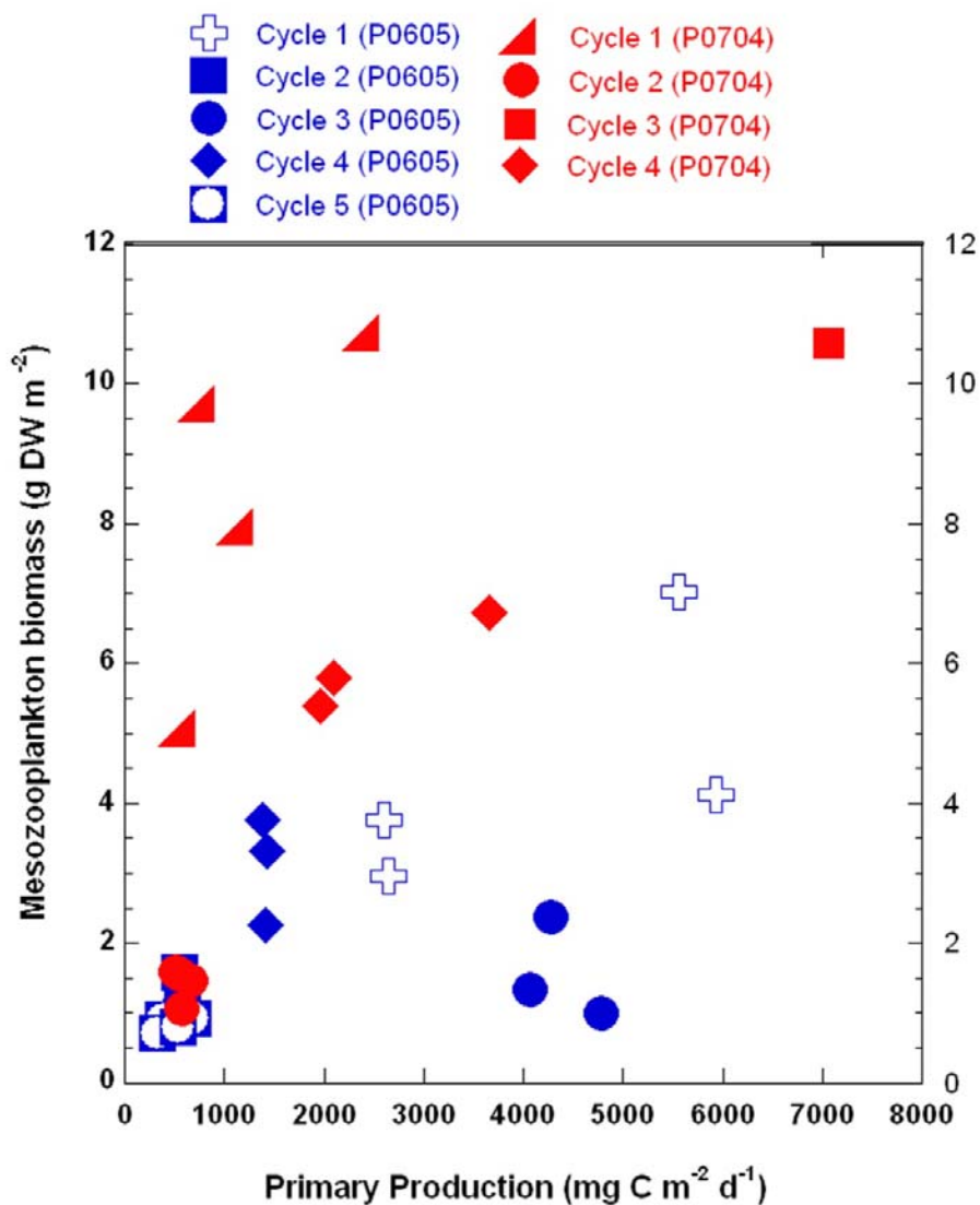
Figure 3.3. Scatter plot of areal estimates of mesozooplankton biomass (g DW m -2 ) against phytoplankton primary production (mg C m -2 d -1 ). Color coding is by cruise, and each experimental cycle is denoted with a different symbol (see legend).
