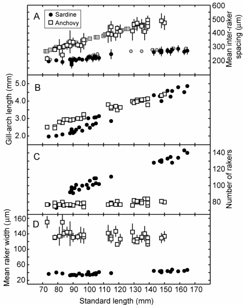
Figure 2.4. Comparison of measures describing the branchial sieves of sardine and anchovy species. A) Black and white symbols represent measurements for species of the CCE, and the solid gray symbols are measurements presented for species of the BCE by King and MacLeod (1976). B) The total length of the first gill arch was taken as the sum of upper- and lower-arch lengths. C) The total number of rakers on the gill arch of sardine continues to increase with fish length over the fish sizes examined, while the number of raker remains fairly constant in anchovy. D) The width of the rakers vary little with fish length. Lines in A and D denote \pm 1 standard deviation.
