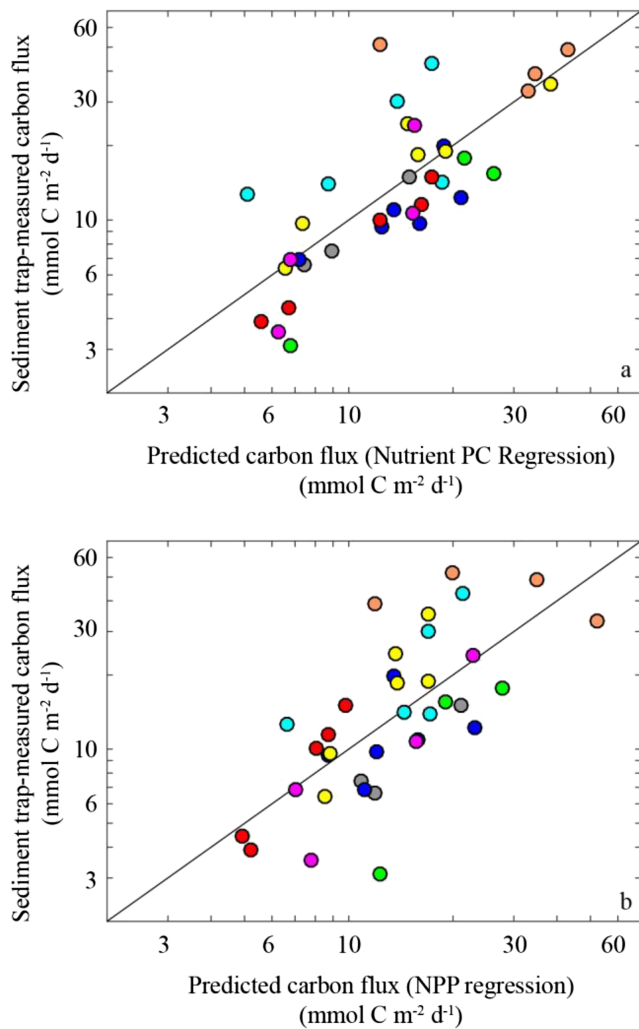
Figure 3. Comparison of sediment trap-measured carbon flux to carbon flux predicted using regressions based on nutrient principal components (a) or NPP (b). OLS regression in (a) is \log_{10}(\text{Export}) = -0.089 \times \text{PC1} + 0.060 \times \text{PC2} + -0.093 \times \text{PC3} + 1.14 . OLS regression in (b) is \log_{10}(\text{Export}) = 0.59 \times \text{NPP} + 0.11 .
