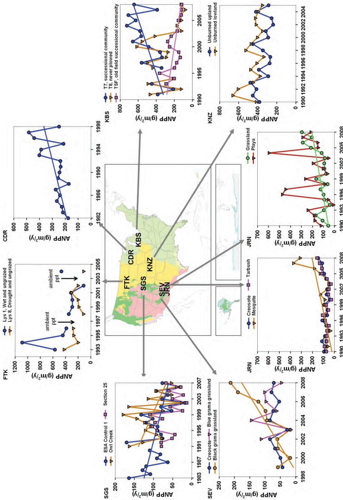
Figure 14-2. Aboveground net primary production (ANPP, g/m 2 /y) for aridland (FTK, JRN, SEV, and SGS) and temperate grassland/savanna (CDR, KBS, and KNZ) sites. A simple linear regression line is displayed if the slope is statistically significant ( p < 0.05 ) and the trend appears linear. The significant slopes are CDR (11), JRN (8, 10), KBS (22, -10), SEV (19), and SGS (-3, -5). Original data from Internet home pages (see table 1-1). Synthesized data from http://www.ecotrends.info .
