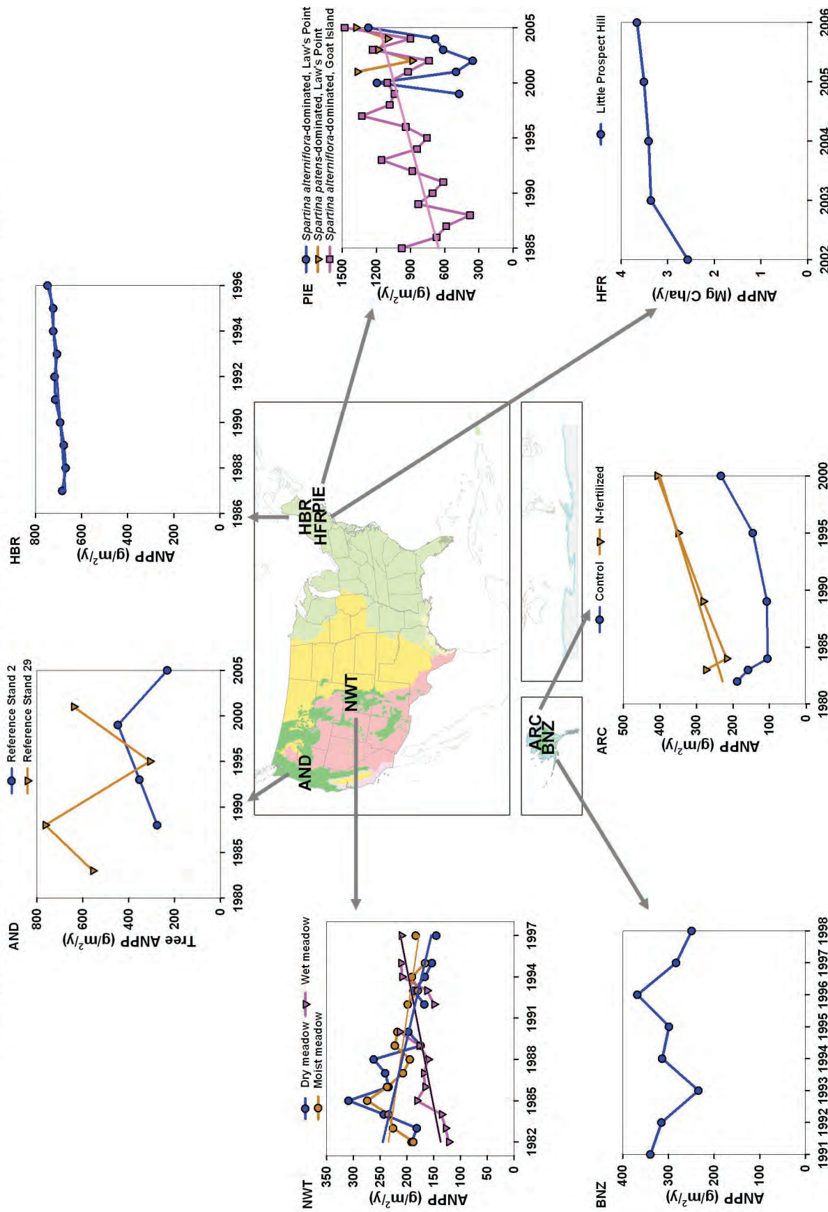
Figure 14-1. Aboveground net primary production (ANPP, g/m 2 /y or Mg C/ha/y) for arctic and alpine (ARC and NWT), coastal (BNZ), eastern and western forest (AND, BNZ, HBR, and HFR) sites. A simple linear regression line is displayed if the slope is statistically significant ( p < 0.05 ) and the trend appears linear. The significant slopes are: ARC (10), HBR (7), NWT (-6, -4, 5), and PIE (-6, -4, 5). Original data from Internet home pages (see table 1-1). Synthesized data from http://www.ecotrends.info .
