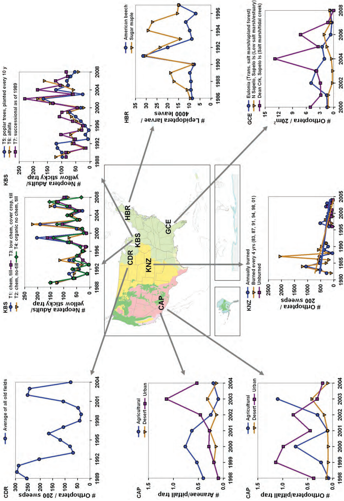
Figure 14-10. Abundance of insects at six sites (CAP, CDR, HBR, GCE, HBR, KBS, and KNZ). A simple linear regression line is displayed if the slope is statistically significant ( p < 0.05 ) and the trend appears linear. The significant slopes are KNZ (-18, -32). Original data from internet home pages (see table 1-1). Synthesized data from http://www.ecotrends.info .
